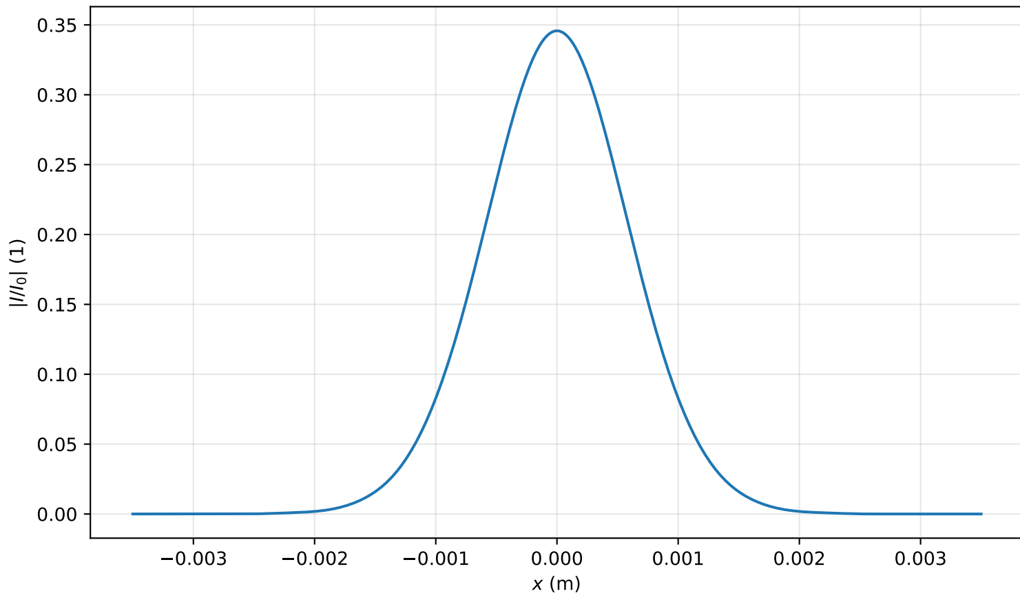
Intensity profile I(x, y = 0, z = 3.184m)/I_0 , P_{in}=0.2P_{cr} , artificial time
